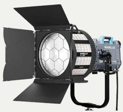
FL-35E Motorized Fresnel Lens 15-46°
